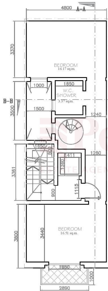
Proposed Fourth Floor Plan
