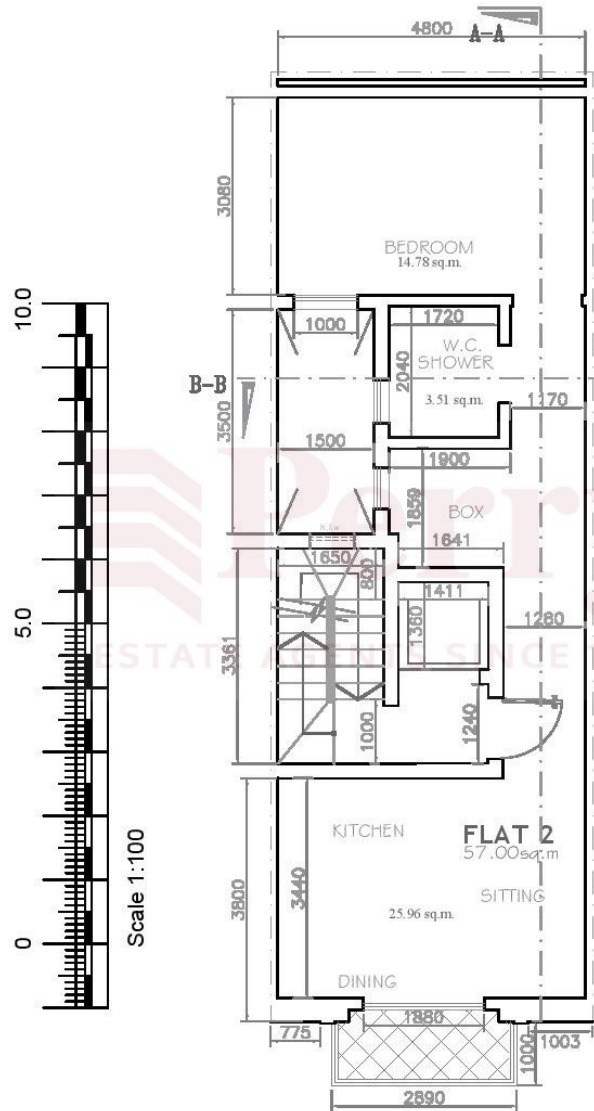
Proposed Second Floor Plan 1:100
