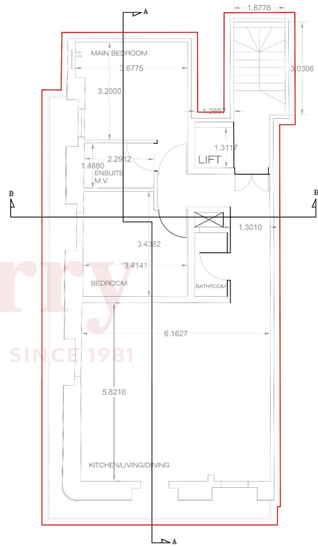
PROPOSED 2ND, 3RD & 4TH FLOORS
