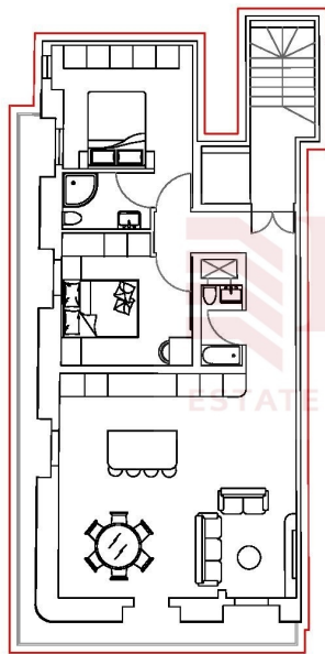
PROPOSED 2ND, 3RD & 4TH FLOORS
