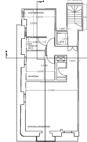
PROPOSED FIRST FLOOR (CLEAN COPY)
