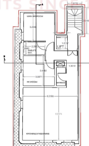
PROPOSED 3RD & 4TH FLOORS
