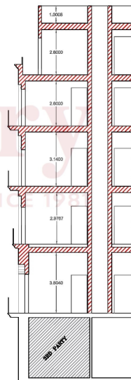
PROPOSED SECTION B-B
