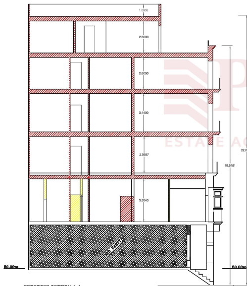
PROPOSED SECTION A-A
