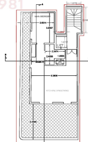
PROPOSED PENTHOUSE LEVEL
