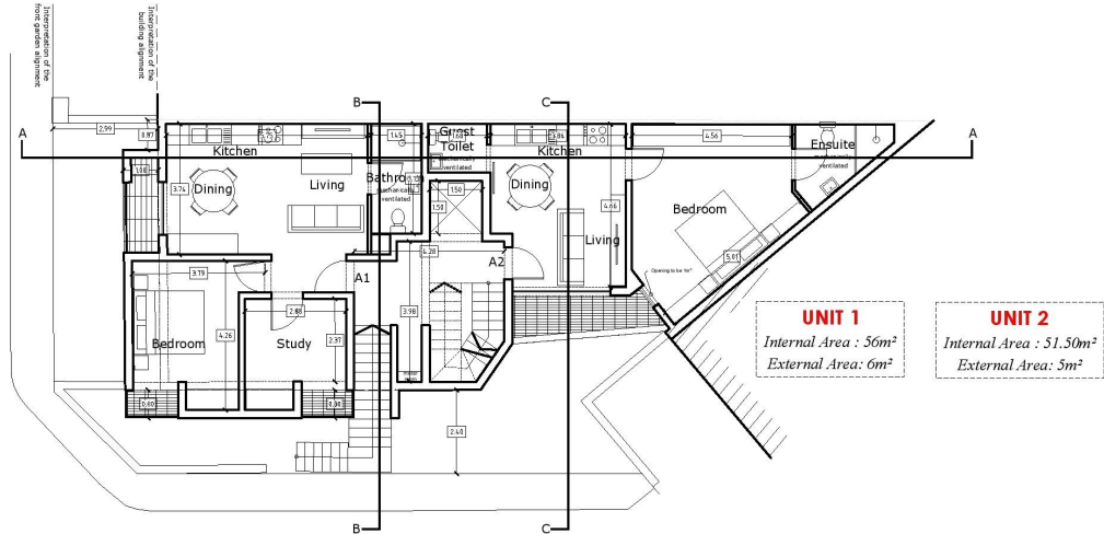
Proposed First Floor Level Scale 1:100
