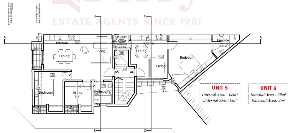
Proposed Third Floor Level Scale 1:100
