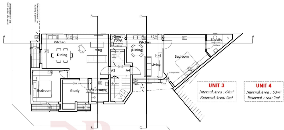
Proposed Second Floor Level Scale 1:100
