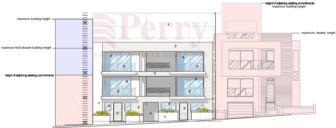
proposed Elevation
