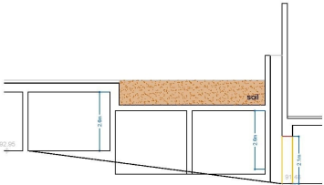
part section x-x through ramp
