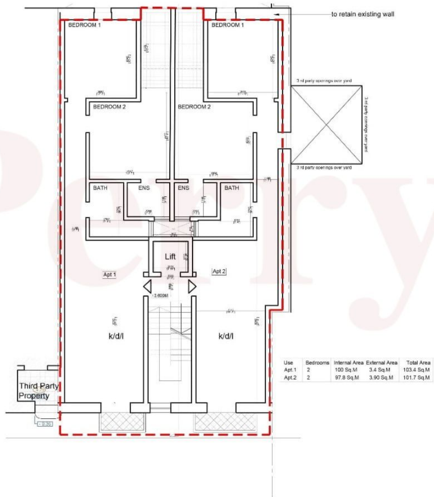
Proposed Level 1
