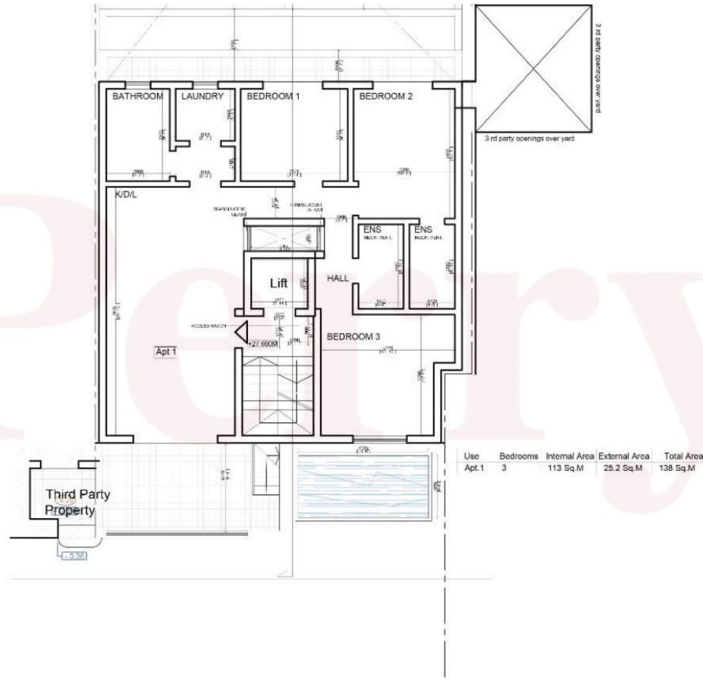
Proposed Level 9
