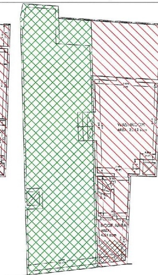
PROPOSED SECOND FLOOR LEVEL (ROOF LEVEL) SCALE 1:100
